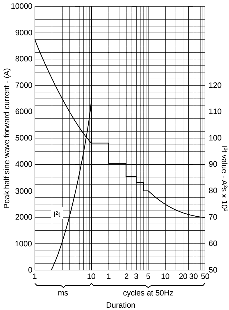
Fig. 3 Surge (non-repetitive) forward current vs time (with 0% V_{RRM} , T_{case} = 150^\circ C )
